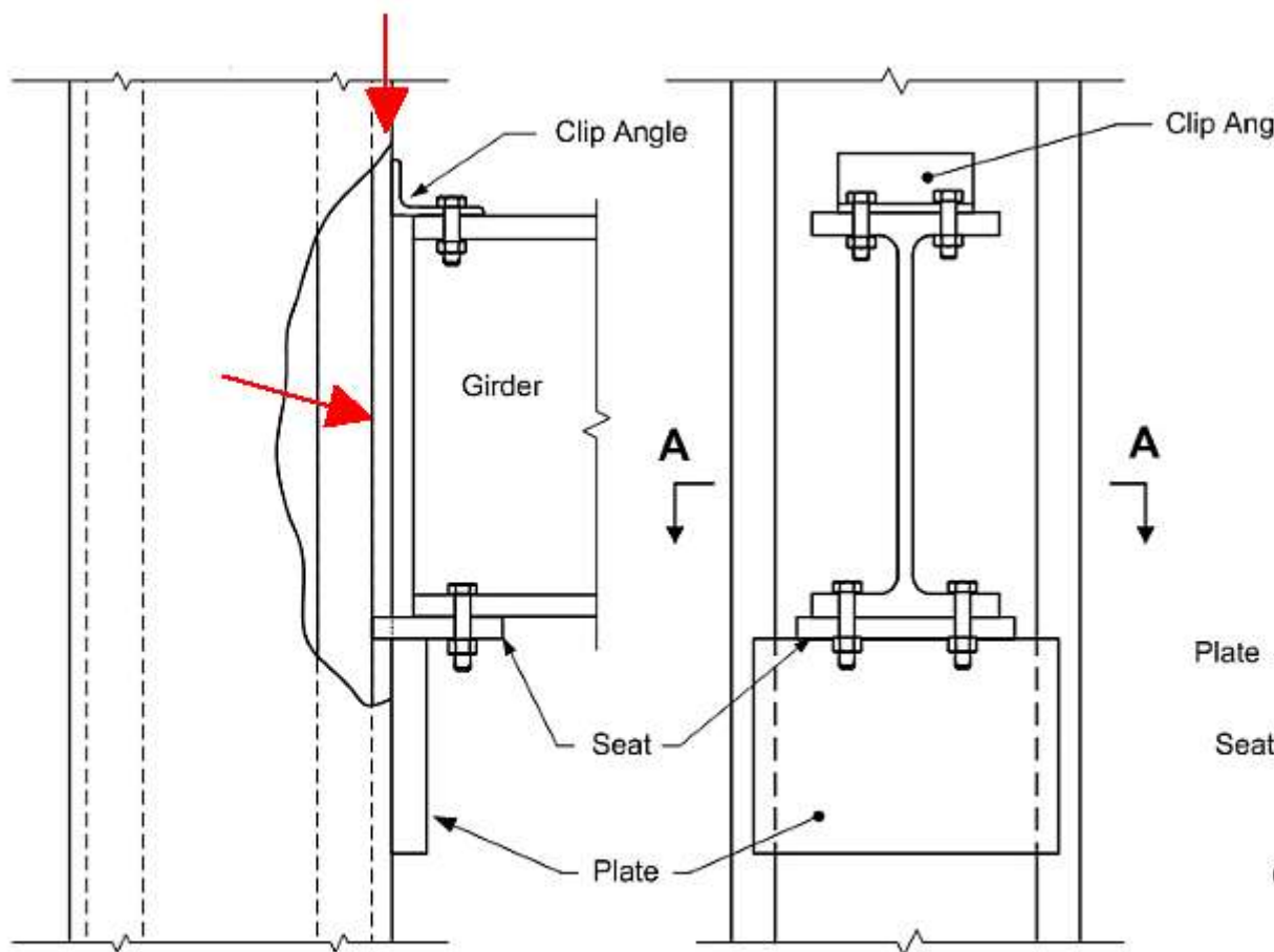
Figure 8–21. Seat connection at Column
